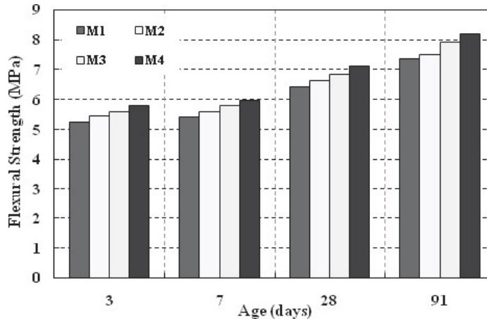
Fig. 4. Flexural strength developments of different concrete mixtures
