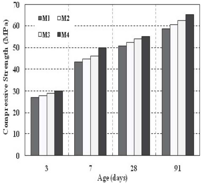
Fig. 2. Compressive strength developments of different concrete mixtures
