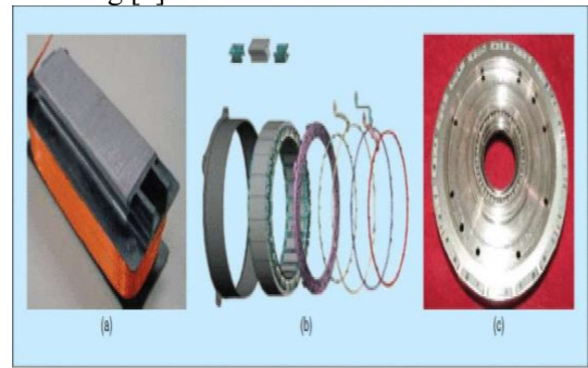
Figure 4 (a) The one-tooth assembly of Chevy Volt's Motor A. (b) Chevy Volt's Motor A assembly diagram. (c) Chevy Volt's Motor A rotor with the end ring removed to show the magnet arrangement [1].
