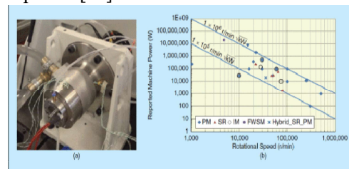
Figure 11 (a) A PM machine with 120,000 r/min and 5 kW under test. (b) The speed–power distribution of reported high-speed generator designs to date.
